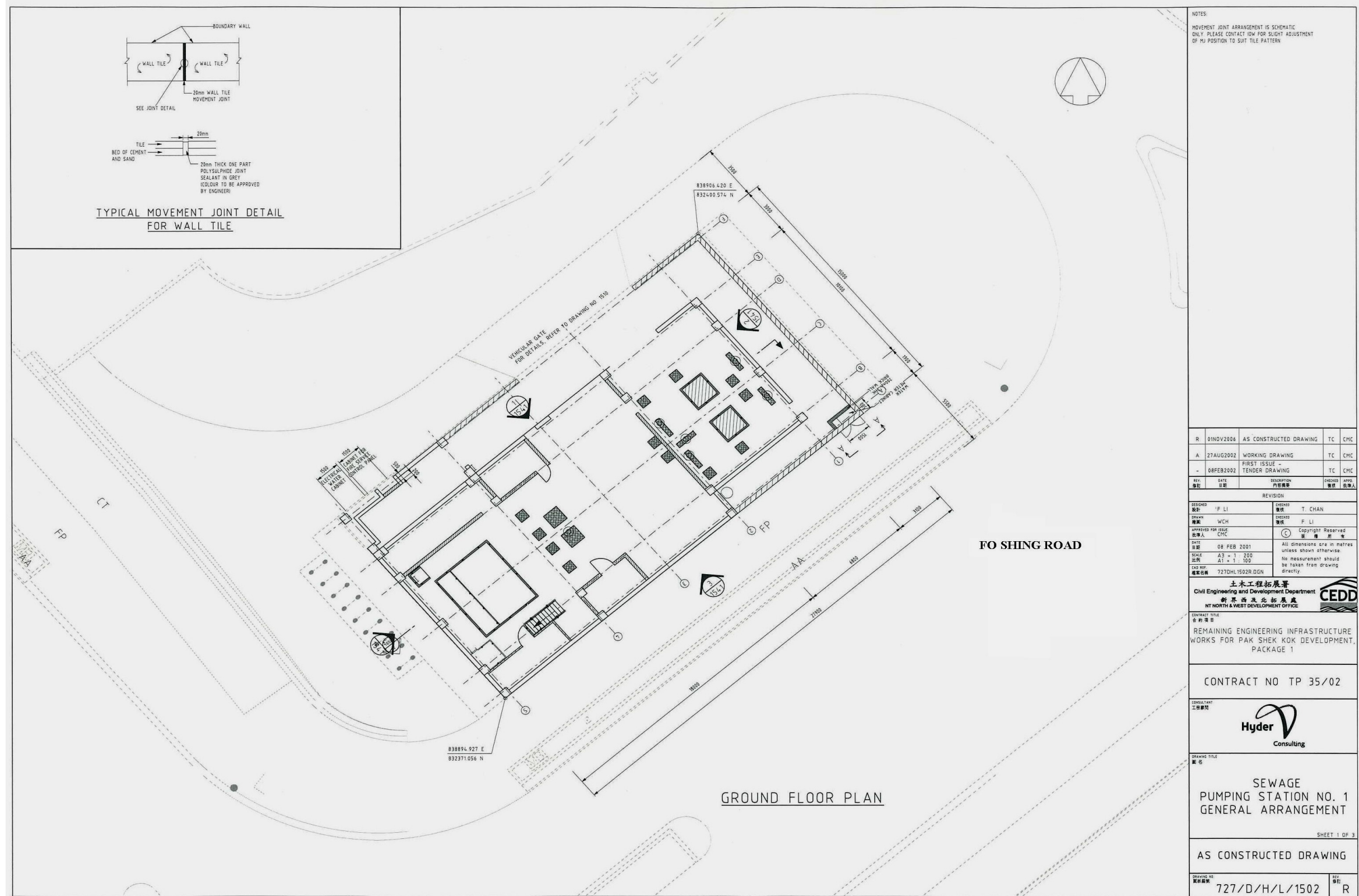
Figure 2: Sewage Pumping Station No. 1 General Arrangement
